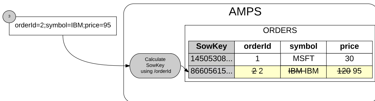
Figure 4.2. Updating the IBM record by matching incoming message keys
