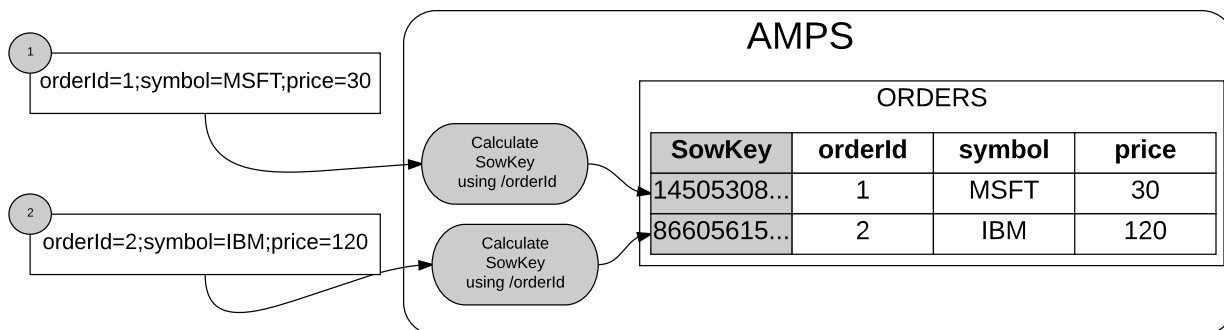
Figure 4.1. A topic named ORDERS recorded in the State of the World with a key definition of /orderId
